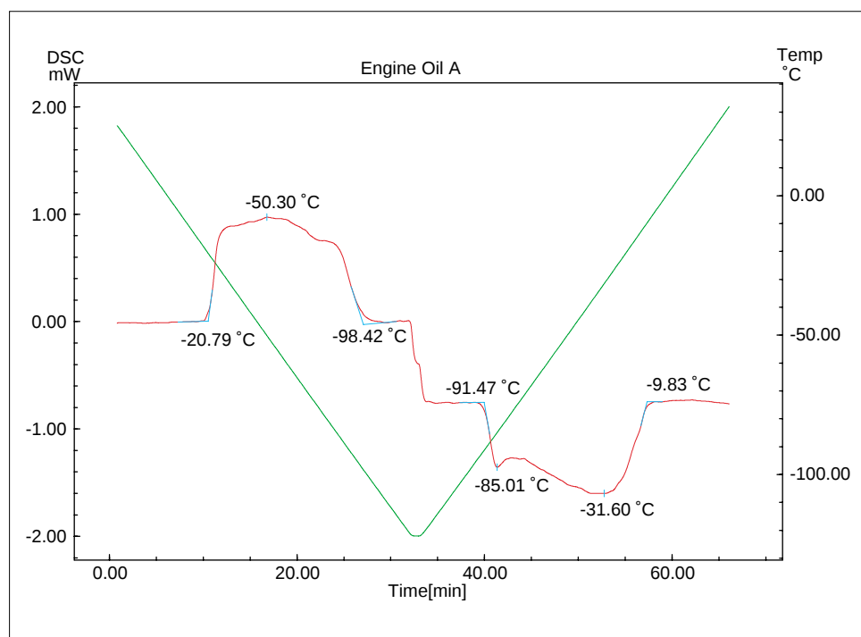
Fig.2 DSC Curve of Engine Oil A
